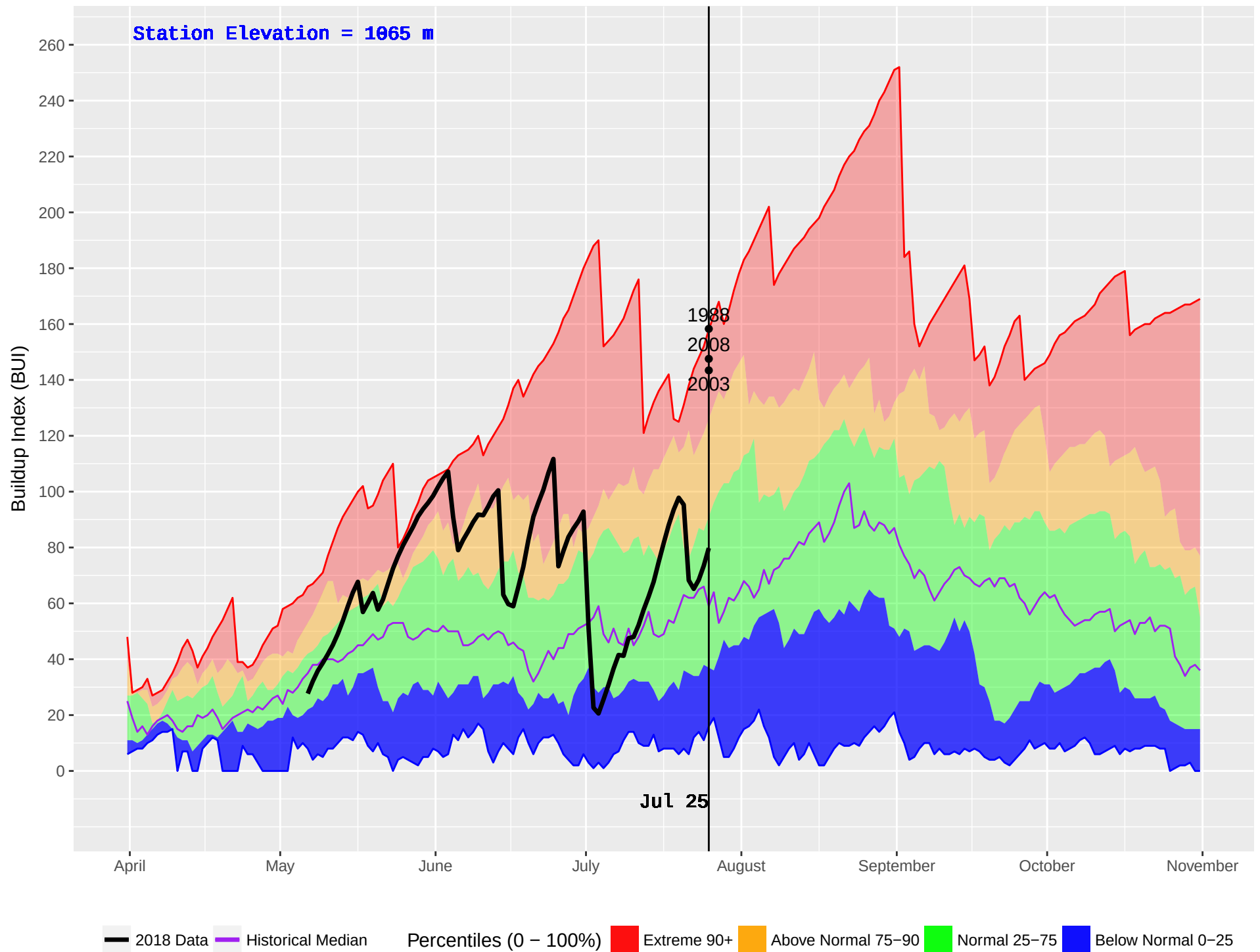
PLACE LAKE (212) : Historical (1981–2016) and Current (2018) Noon Buildup Index (BUI)
