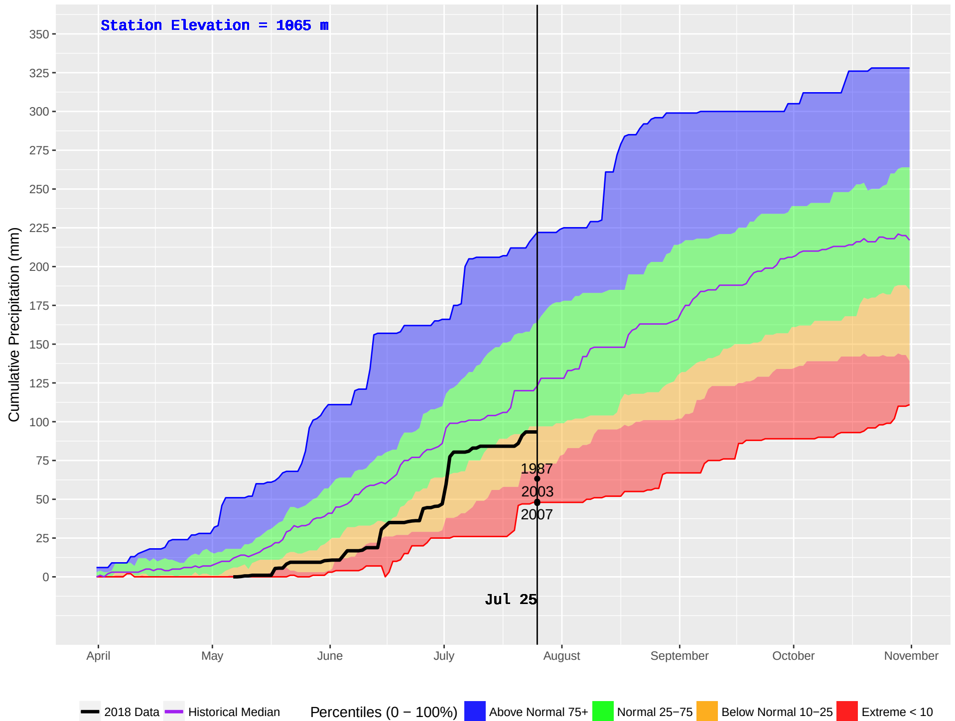
PLACE LAKE (212) : Historical (1981–2016) and Current (2018) Noon Cumulative Precipitation
