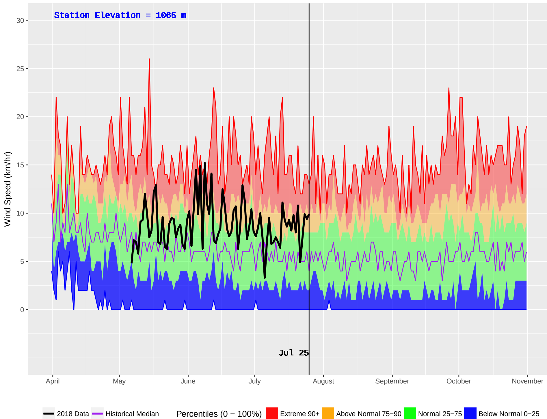
PLACE LAKE (212) : Historical (1981–2016) and Current (2018) Noon Wind Speed
