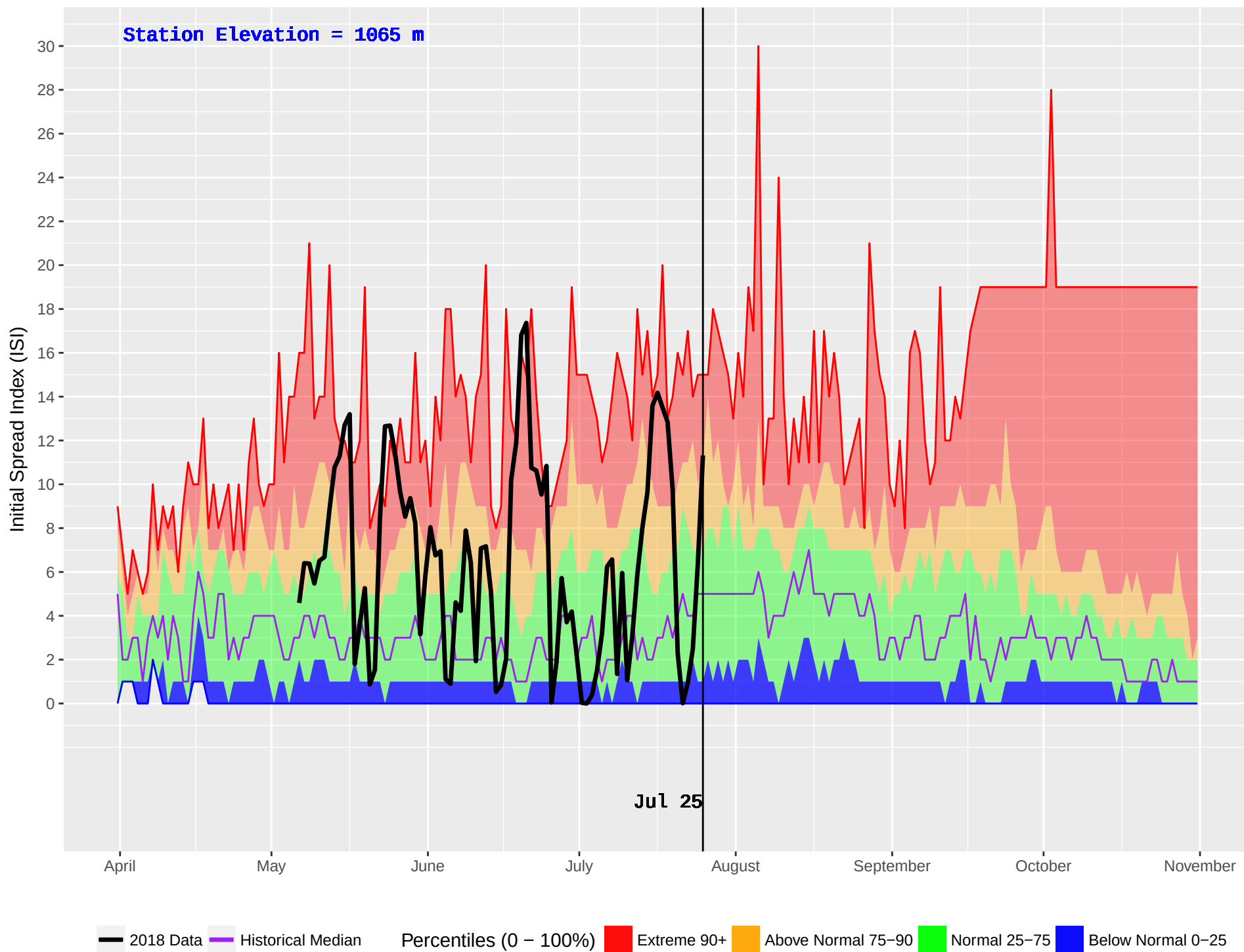
PLACE LAKE (212) : Historical (1981–2016) and Current (2018) Noon Initial Spread Index (ISI)
