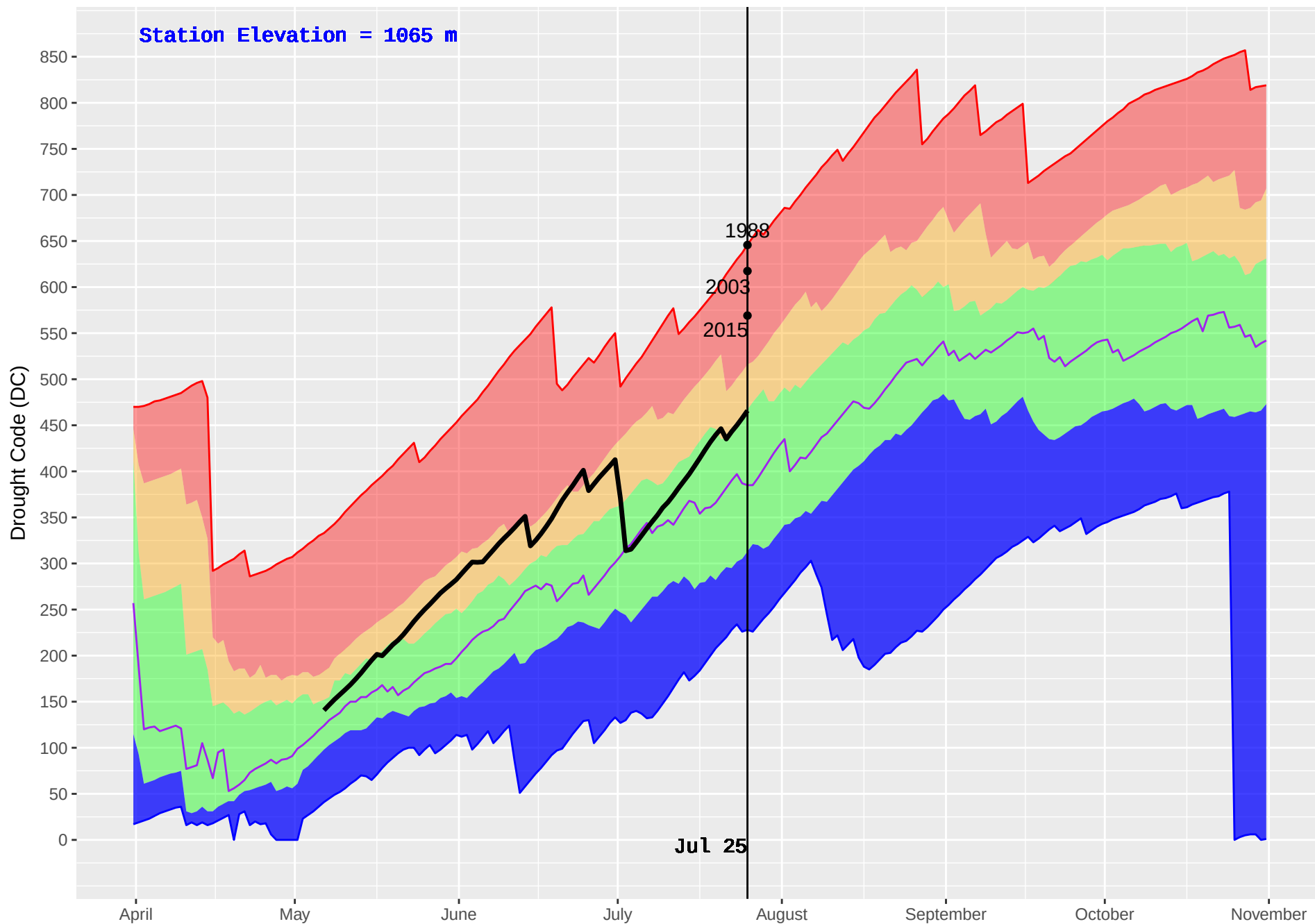
PLACE LAKE (212) : Historical (1981–2016) and Current (2018) Noon Drought Code (DC)
