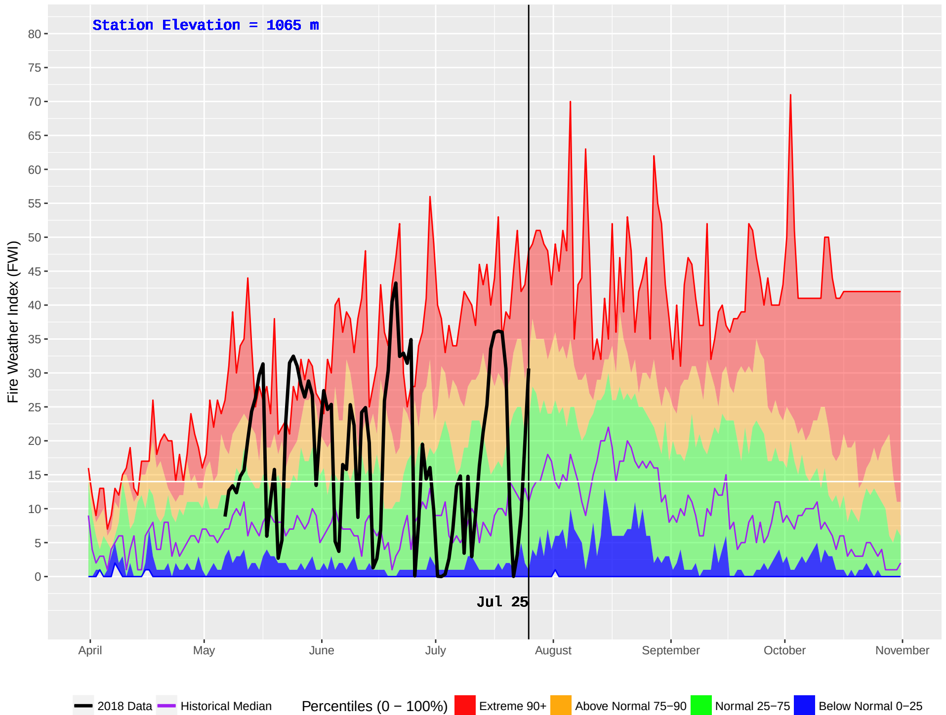
PLACE LAKE (212) : Historical (1981–2016) and Current (2018) Noon Fire Weather Index (FWI)
