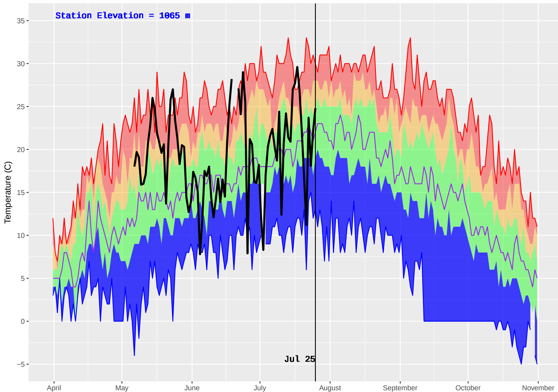
PLACE LAKE (212) : Historical (1981–2016) and Current (2018) Noon Temperature
